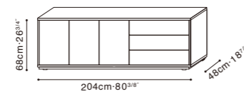
C0400219 Cabinet
