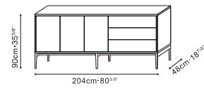
C0400210 Cabinet High Version
