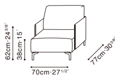
C01H0101 Chair
